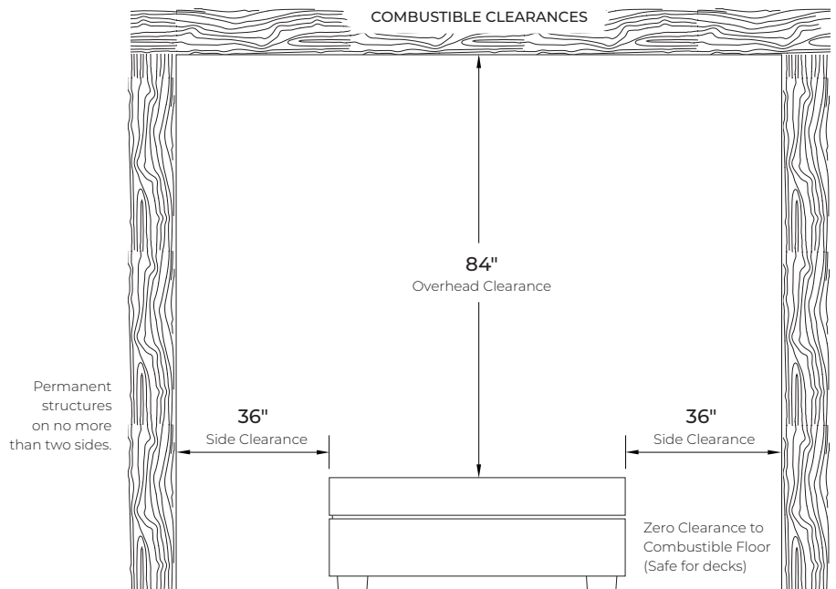
CROSS SECTION
